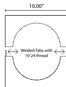
ANCHOR PLATE
